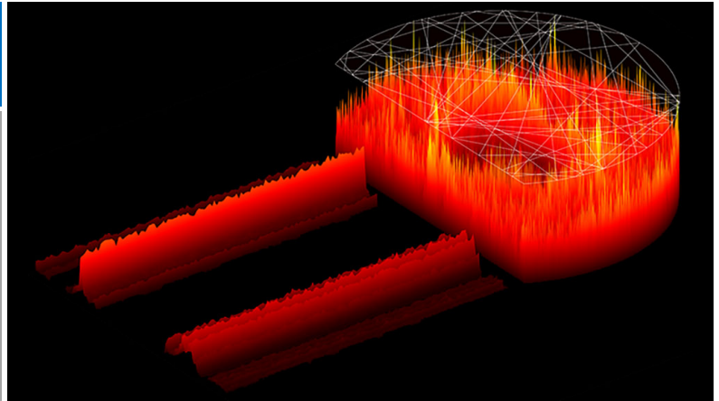
Stable emission from a D-Shaped semiconductor laser - Hui Cao Group
