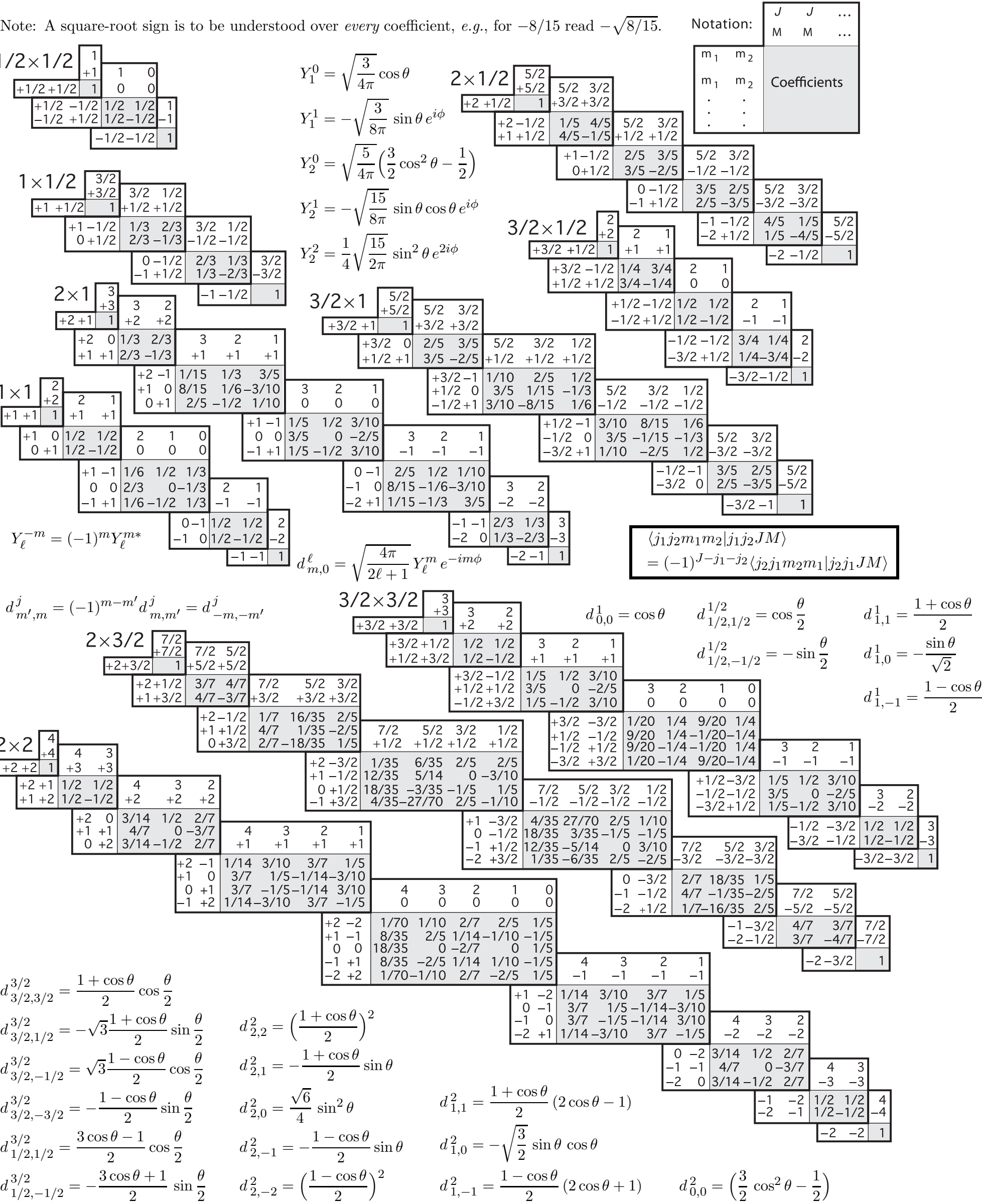
Figure 44.1: The sign convention is that of Wigner ( Group Theory , Academic Press, New York, 1959), also used by Condon and Shortley ( The Theory of Atomic Spectra , Cambridge Univ. Press, New York, 1953), Rose ( Elementary Theory of Angular Momentum , Wiley, New York, 1957), and Cohen ( Tables of the Clebsch-Gordan Coefficients , North American Rockwell Science Center, Thousand Oaks, Calif., 1974).
